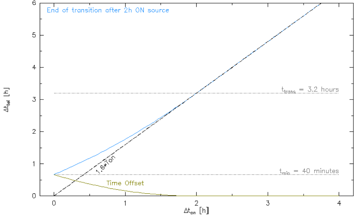
Figure 4: Relation between \Delta t_{\text{tel}} and \Delta t_{\text{on}} as implemented in ASTRO and PMS sensitivity estimators
